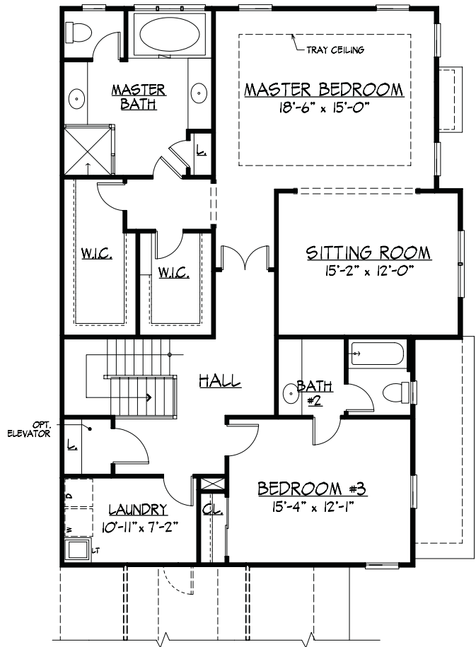
Optional Second Floor Plan
